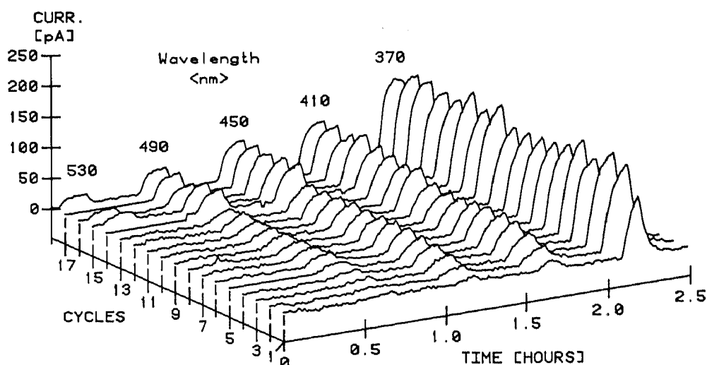
Fig. 3. Self-sensitization experiment of an aqueous \text{Ag}^+ zeolite A dispersion. (1 nA s corresponds to 6.82 nl of oxygen.)
