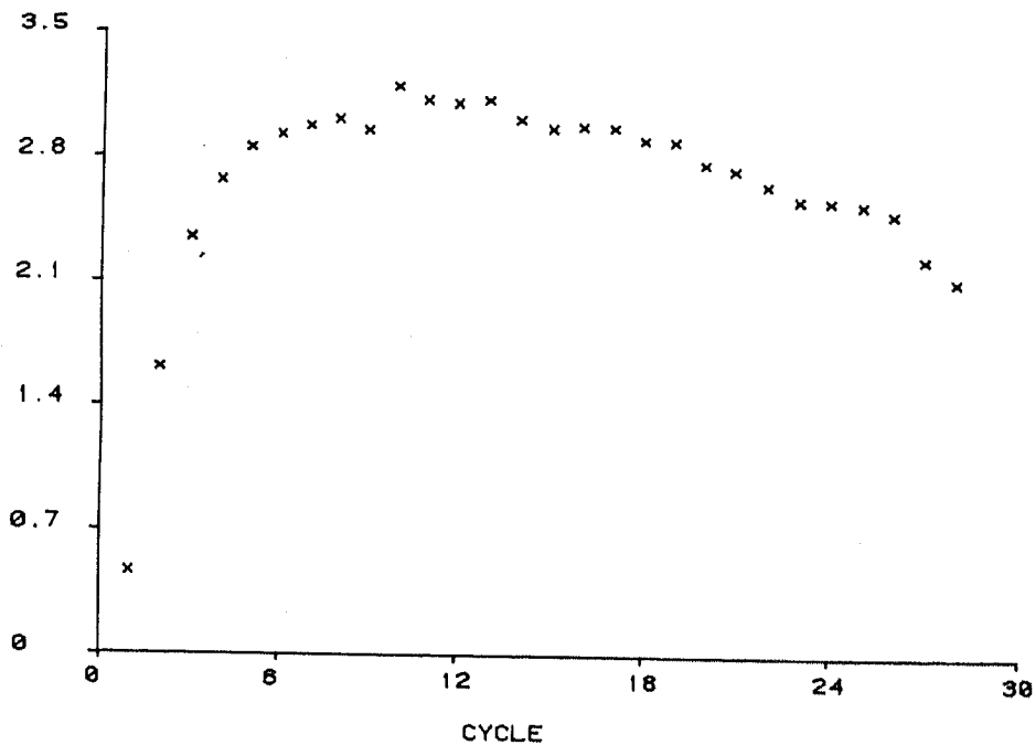
Fig. 5. (a) Oxygen produced at various wavelengths in each cycle vs. the cycle number (+, 370 nm; O, 410 nm; Δ, 450 nm; ◇, 490 nm; □, 530 nm); (b) oxygen produced in a complete cycle vs. the cycle number.
