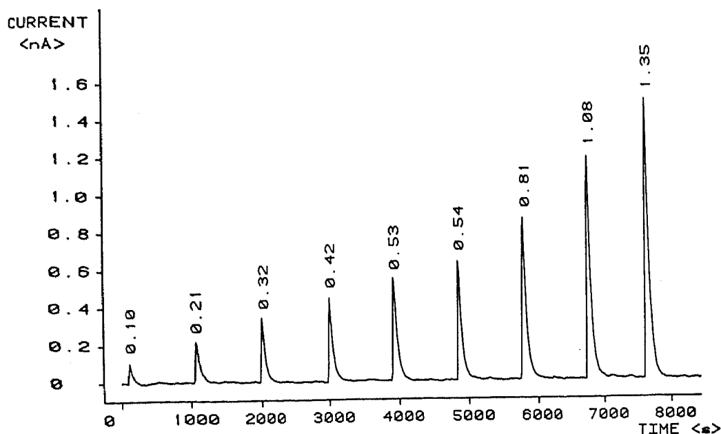
Fig. 8. Calibration signals of the Clark electrode. (The numerals on each peak indicate the number of microlitres of oxygen.)
