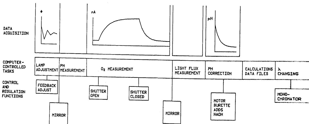
Fig. 7. Experimental flow at each wavelength.
