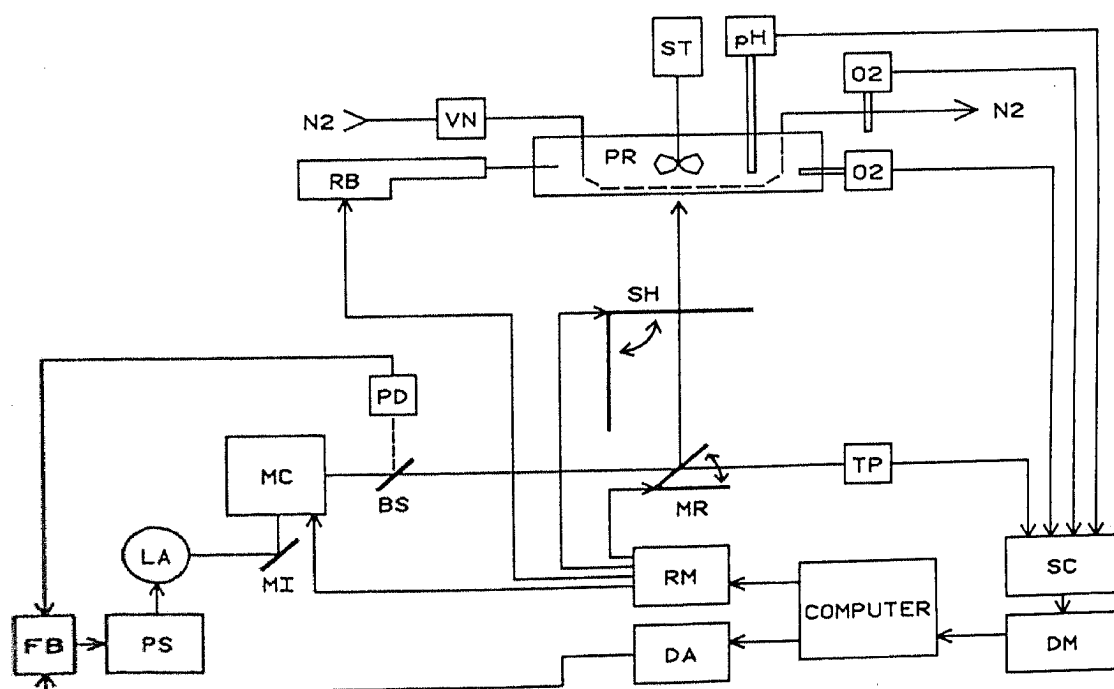
Fig. 6. Experimental set-up (see text).
