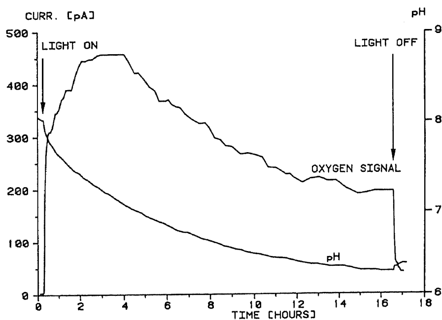
Fig. 2. Photo-oxygen generation and corresponding pH dependence of an aqueous \text{Ag}^+ zeolite A. The total oxygen evolution in this experiment was 463 \mu\text{l} .
