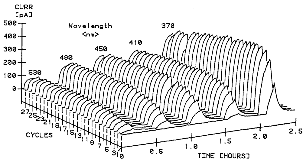
Fig. 4. Self-sensitization experiment of an aqueous \text{Ag}^+ zeolite A dispersion. (1 nA s corresponds to 3.94 nl of oxygen.)
