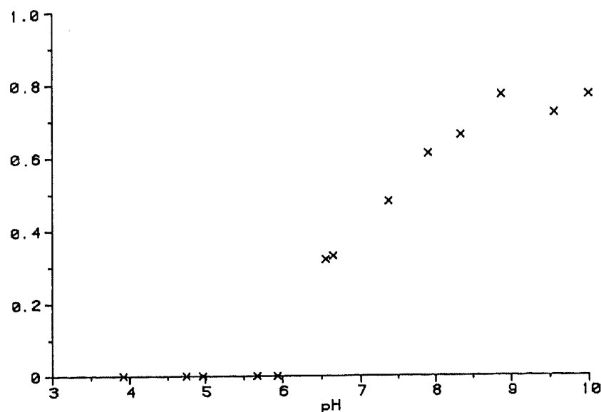
Fig. 1. pH dependence of photo-oxygen evolution of an aqueous dispersion of \text{Ag}^+ mordenite.
